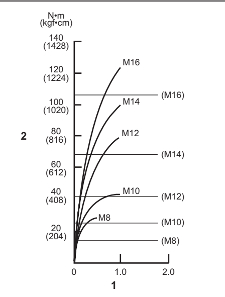
1. Fastening time (second) 2. Fastening torque
